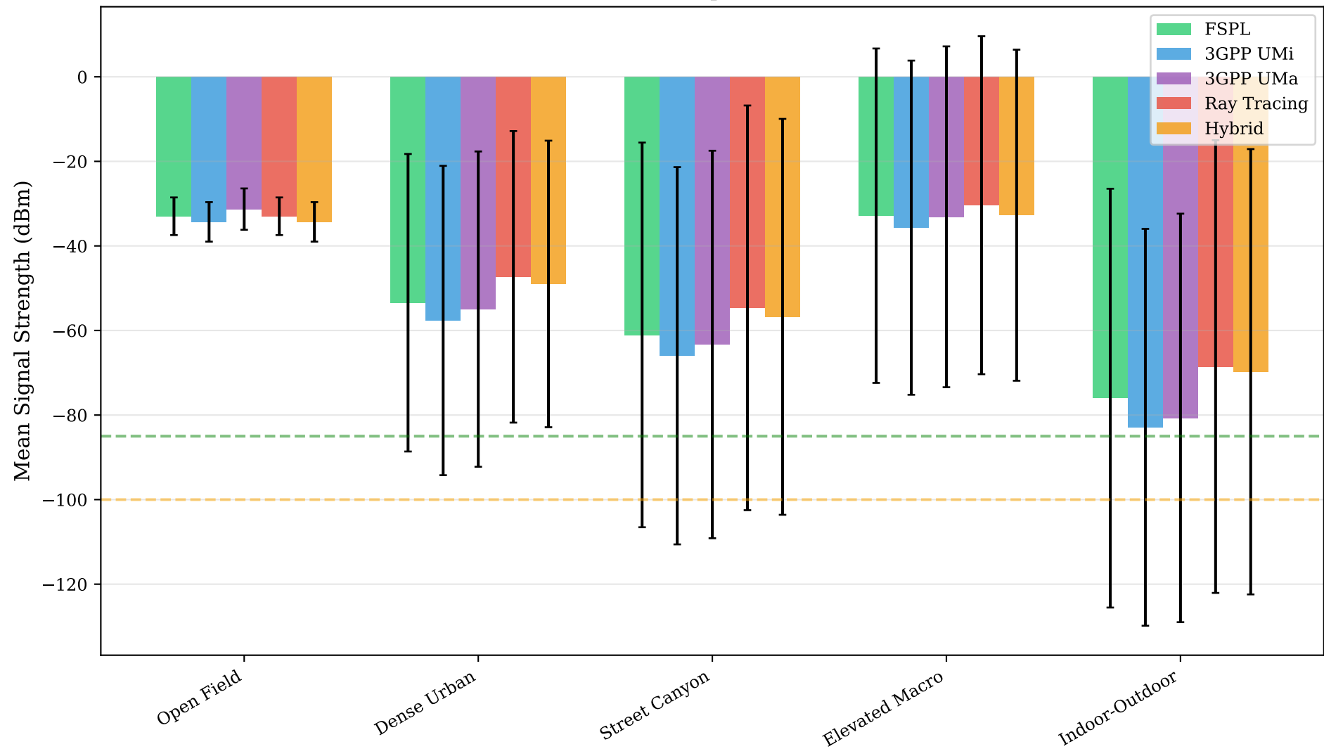
Model Performance Comparison Across Scenarios
