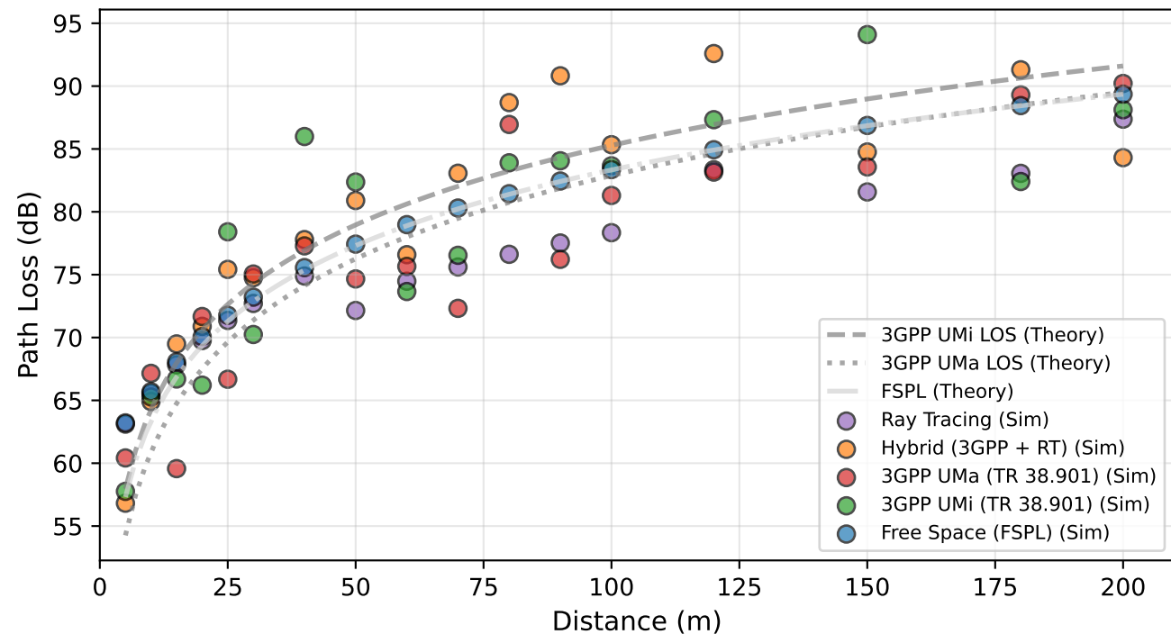
Path Loss vs Distance (LOS)
