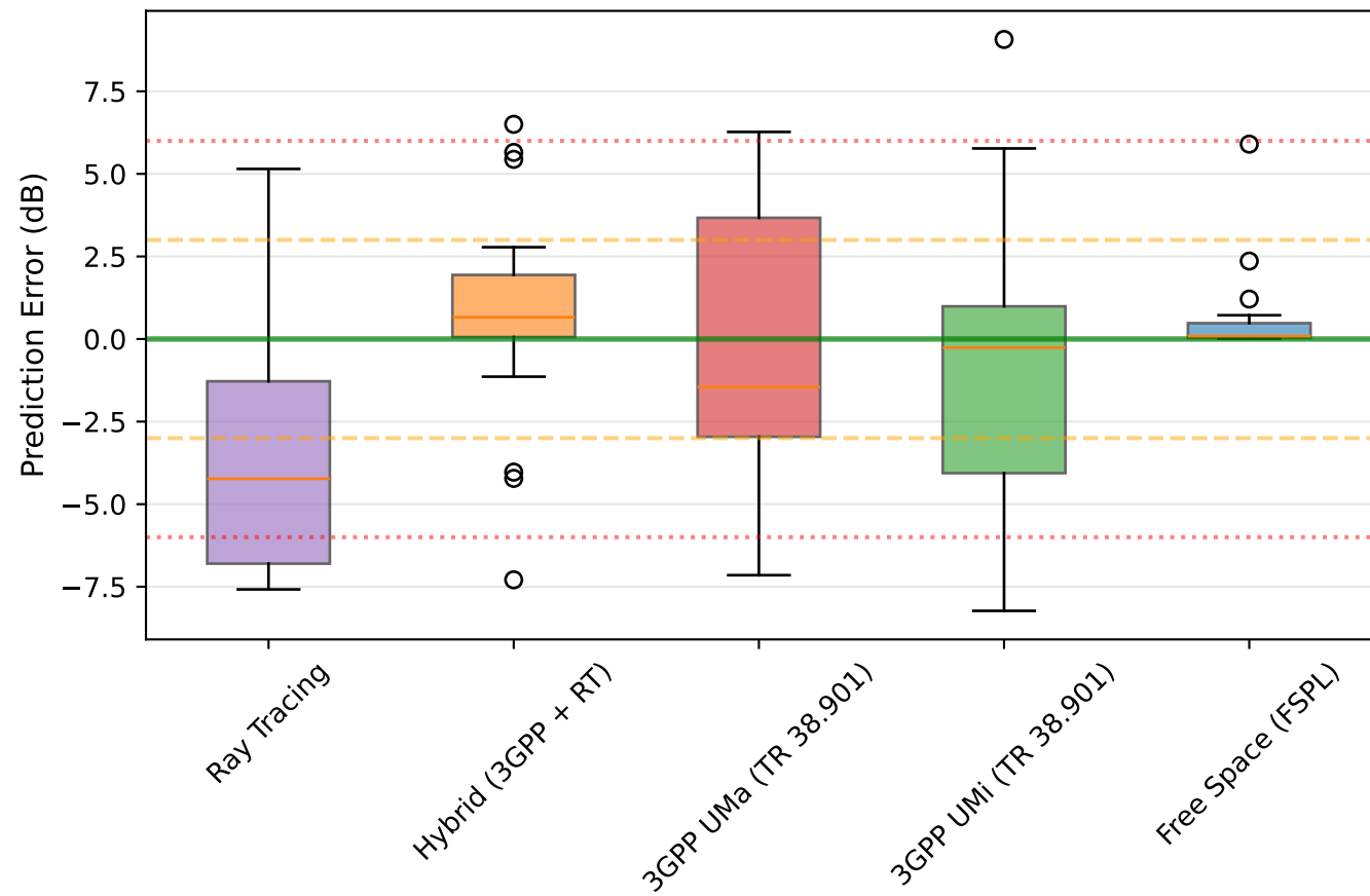
Error Distribution (LOS)
