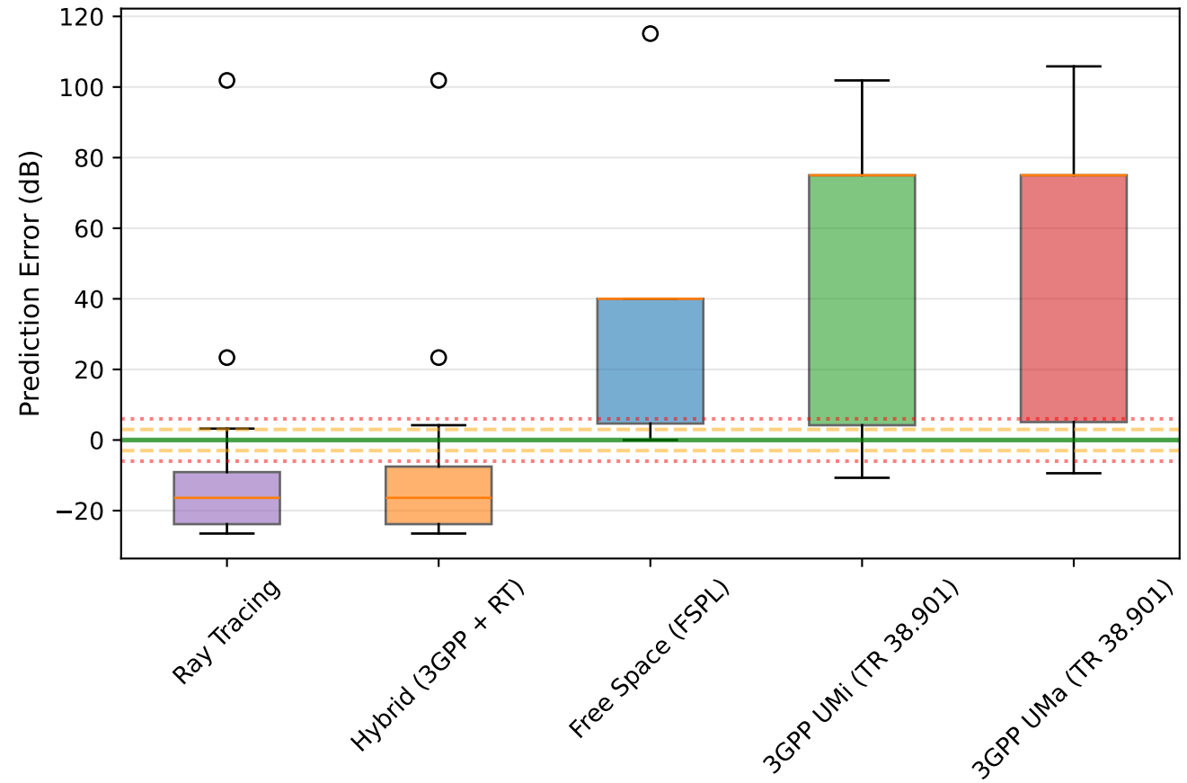
Error Distribution (NLOS)
