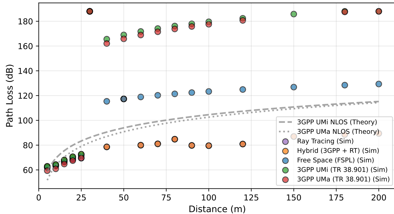
Path Loss vs Distance (NLOS)
