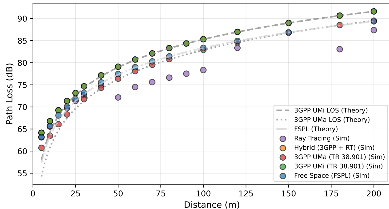
Path Loss vs Distance (LOS)
