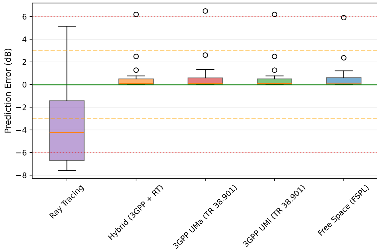
Error Distribution (LOS)
