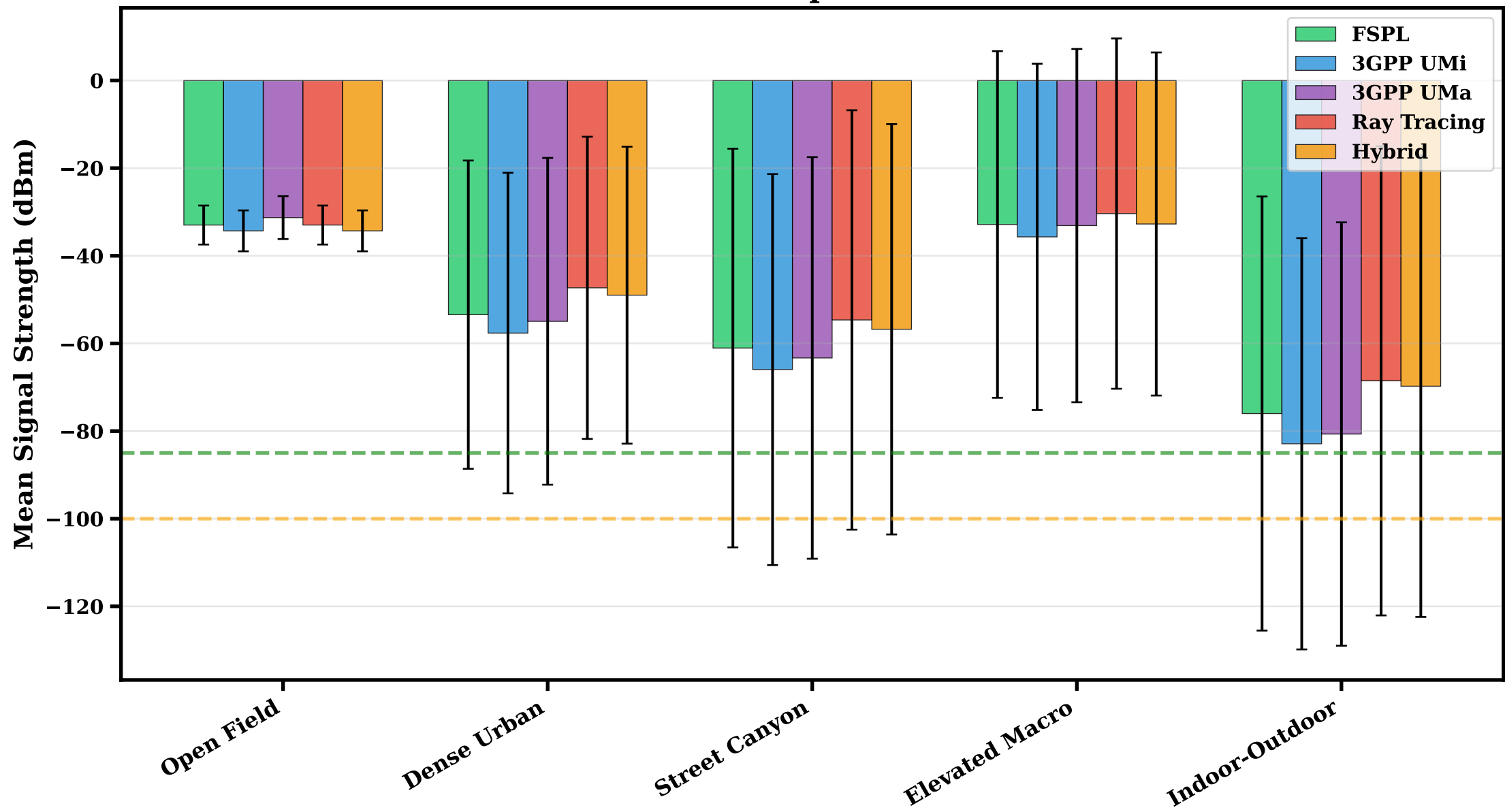
Model Performance Comparison Across Scenarios
