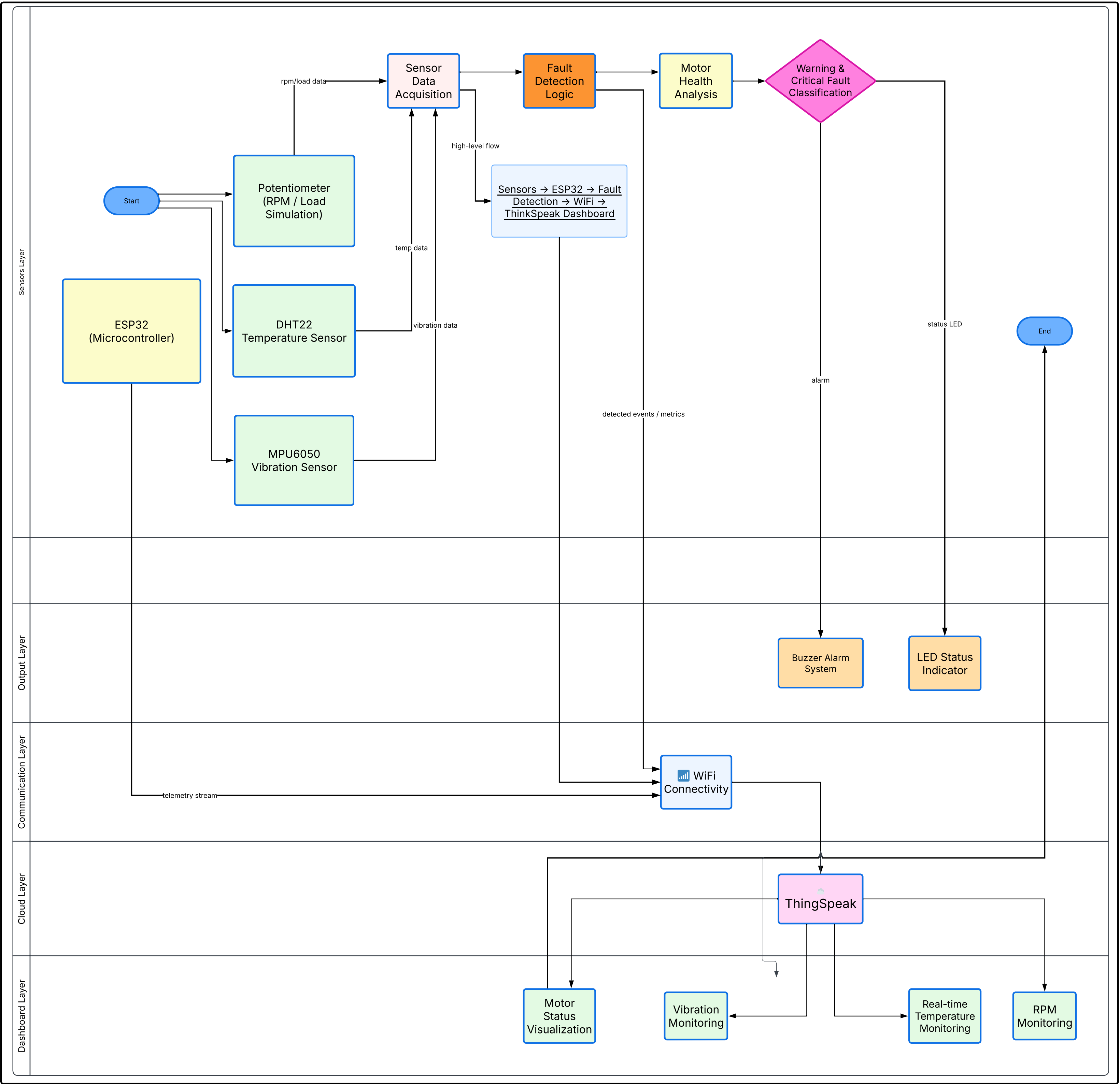
IoT-Based Industrial Motor Health Monitoring System Architecture
