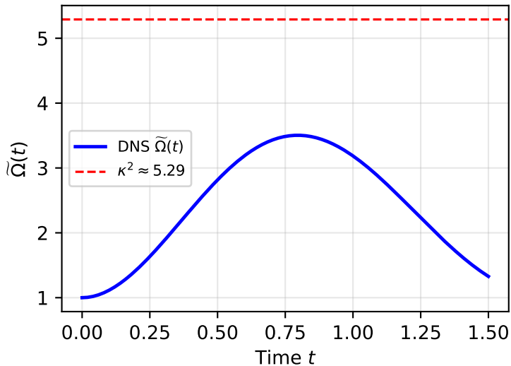
Enstrophy Boundedness
