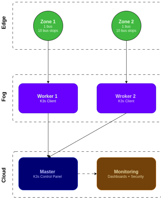
Figure 1: System architecture
