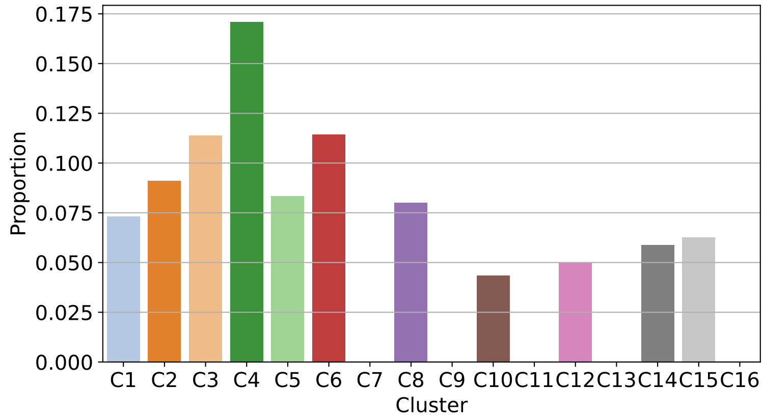
Obesity proportion by cluster
