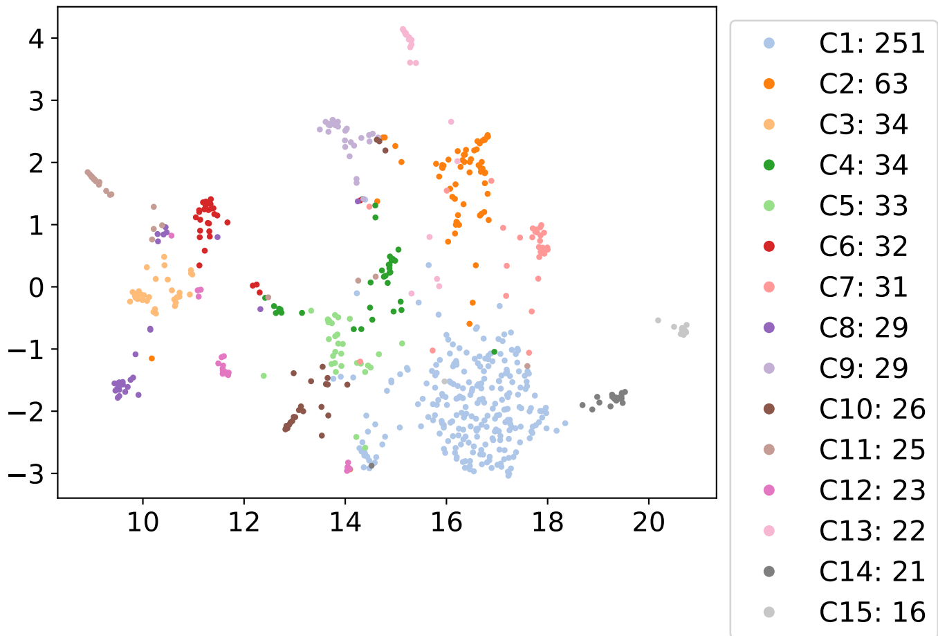
minibatch 15 clusters
