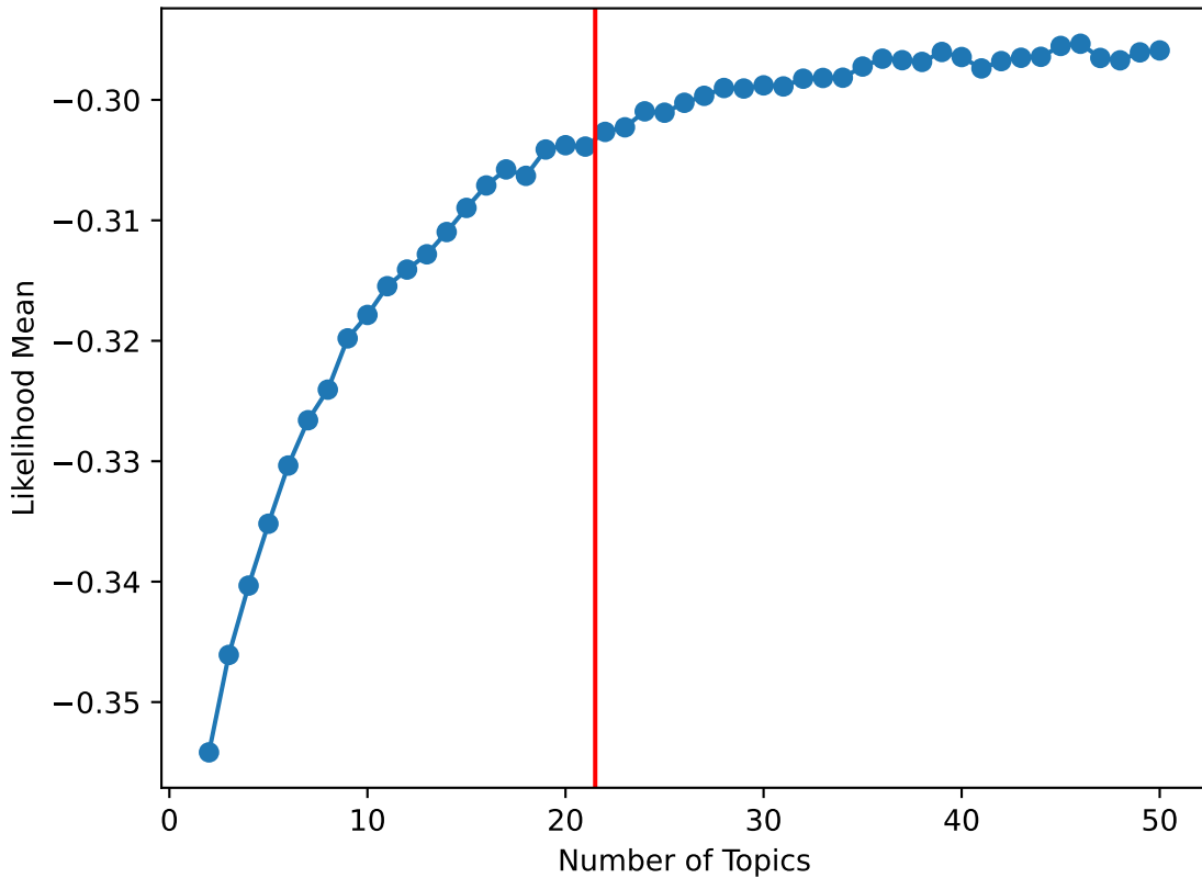
Data Likelihood (average of 10 runs)
