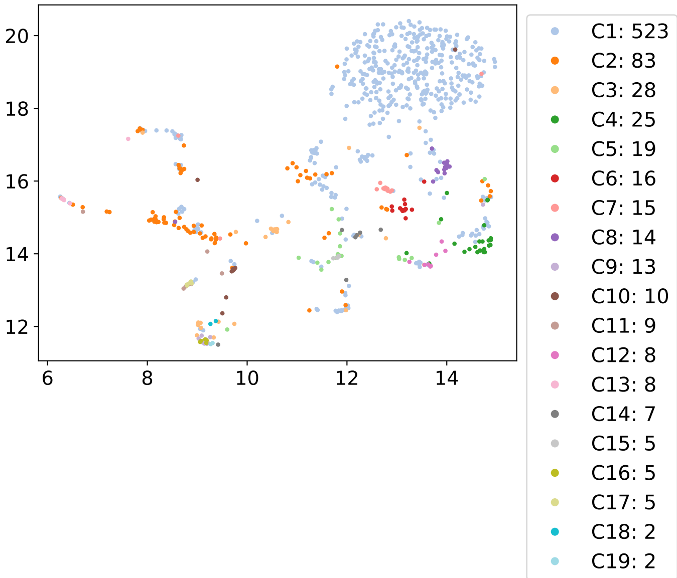
kmeans 19 clusters
