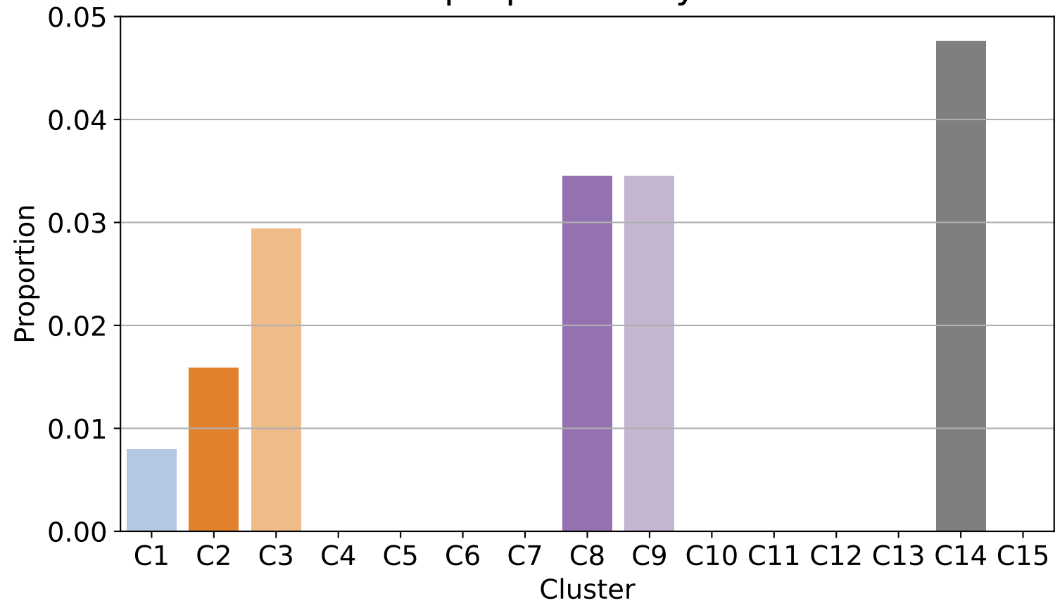
venti proportion by cluster
