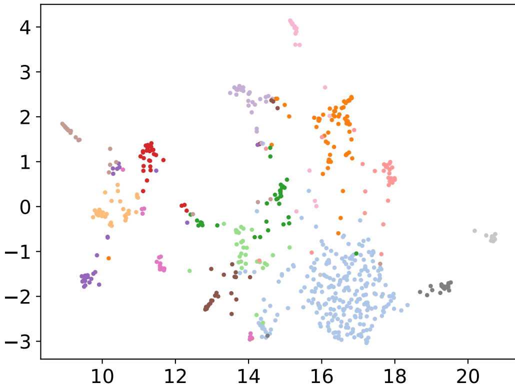
minibatch 15 clusters
