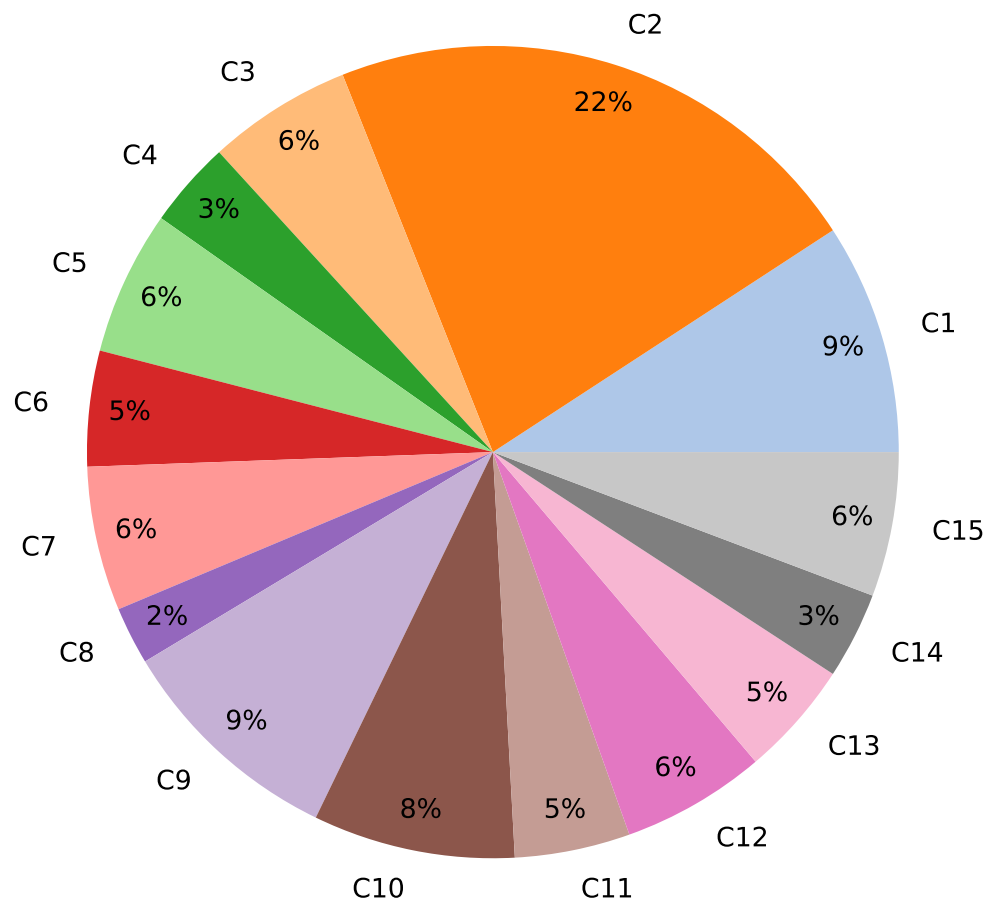
Cluster Composition for increasing EQ5D (recovered)
