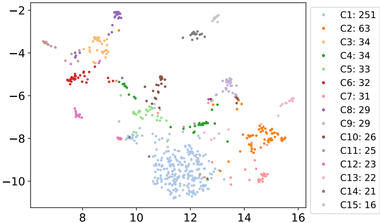
minibatch 15 clusters
