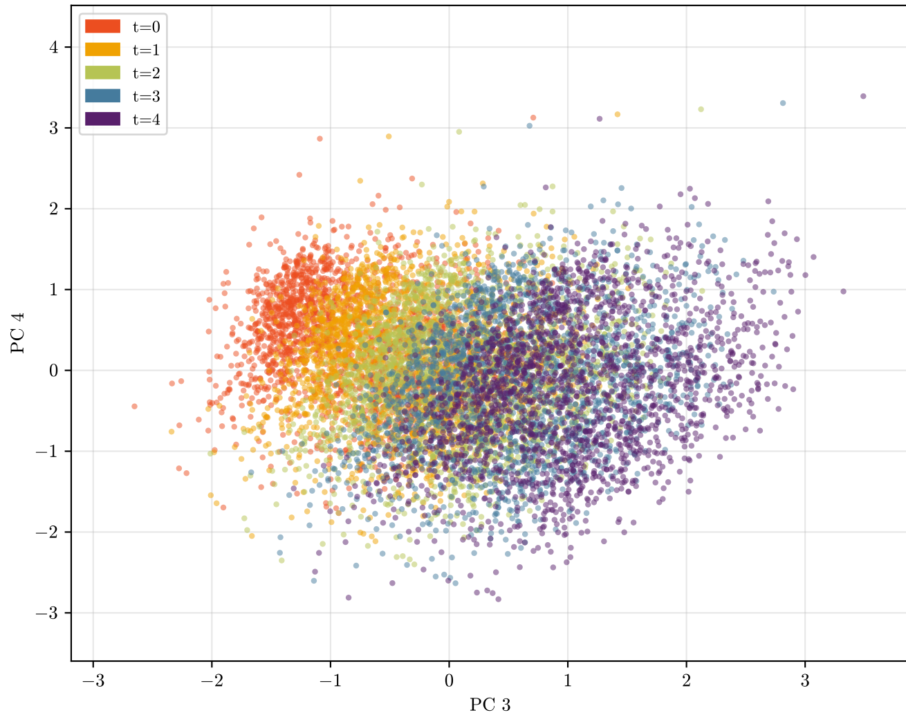
Learned Trajectories
