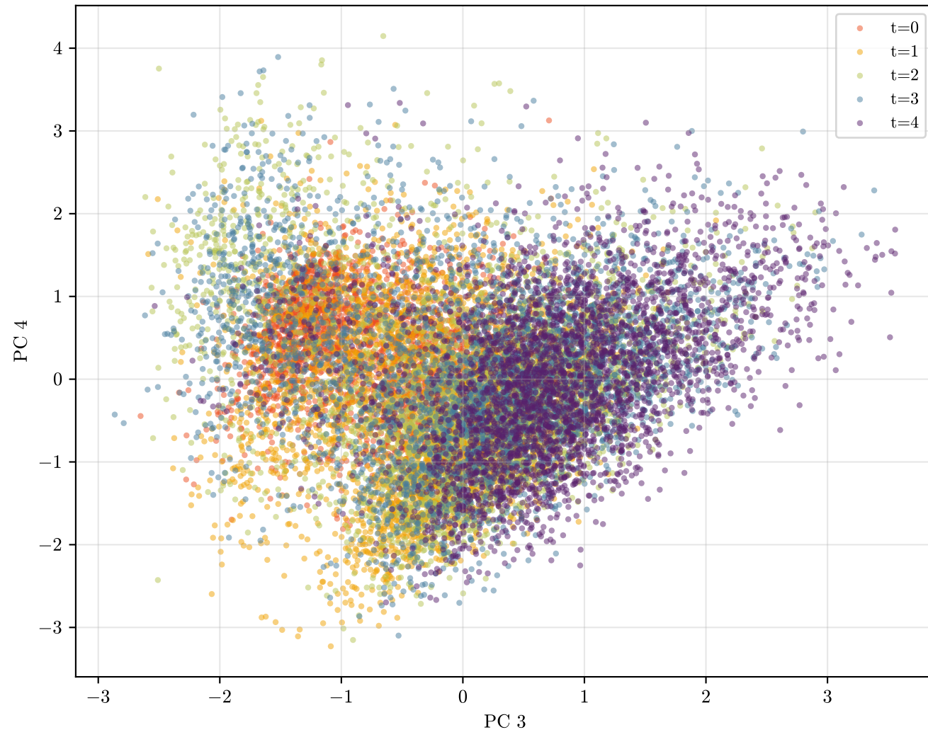
Ground Truth Marginals
