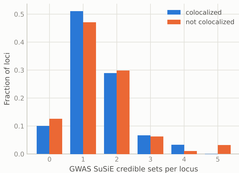
C Allelic heterogeneity (multi-CS Fisher p=0.9 )
