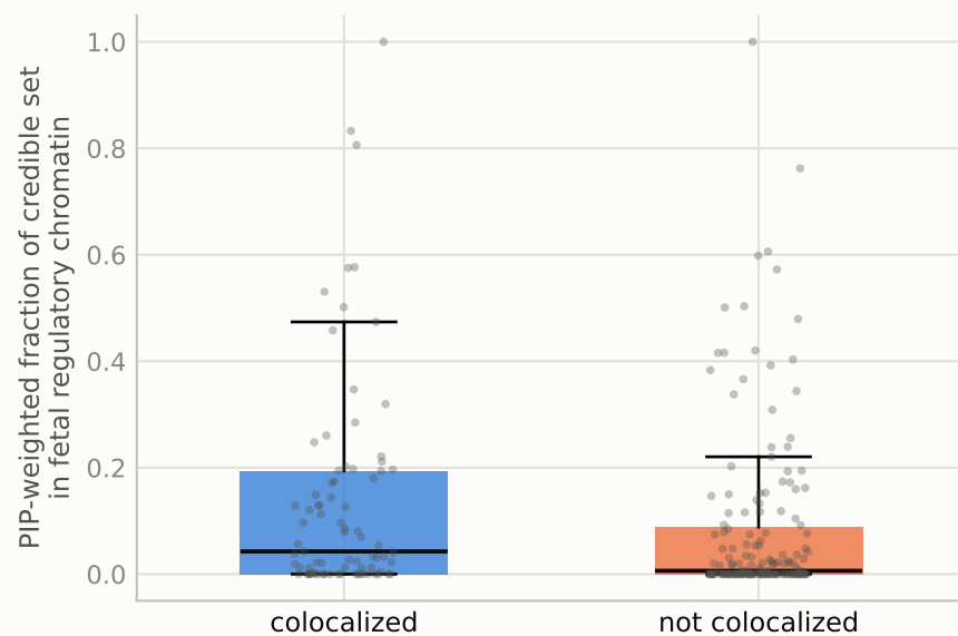
D Fetal regulatory annotation (MWU p=0.0013 )
