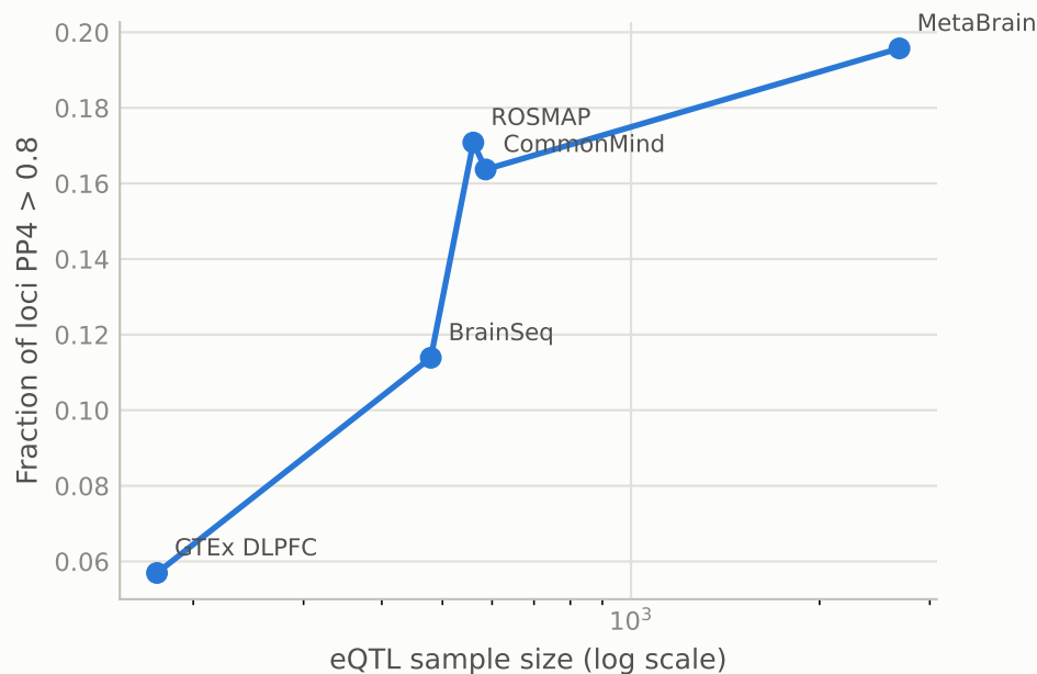
A Power: OR 2.5 per 10× eQTL N ( p=3.8\text{e-}06 )
