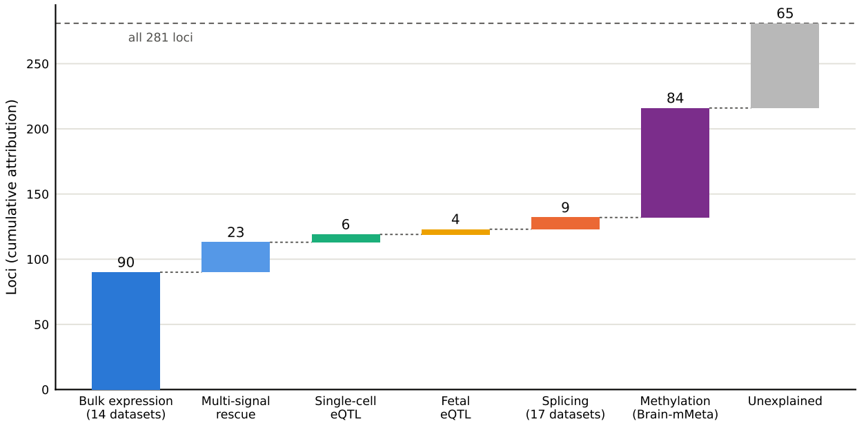
Sequential attribution of 281 schizophrenia loci across molecular channels (PP4 > 0.8)
