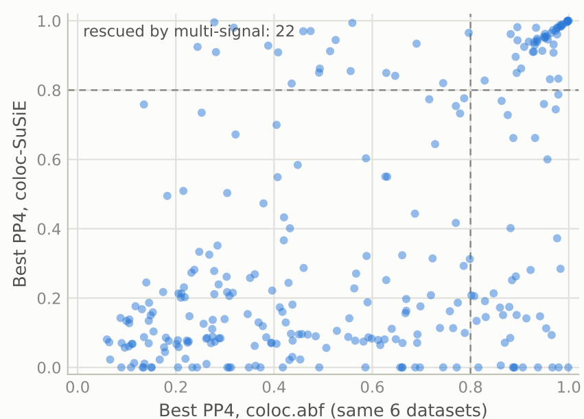
B Single-variant vs multi-signal colocalization
