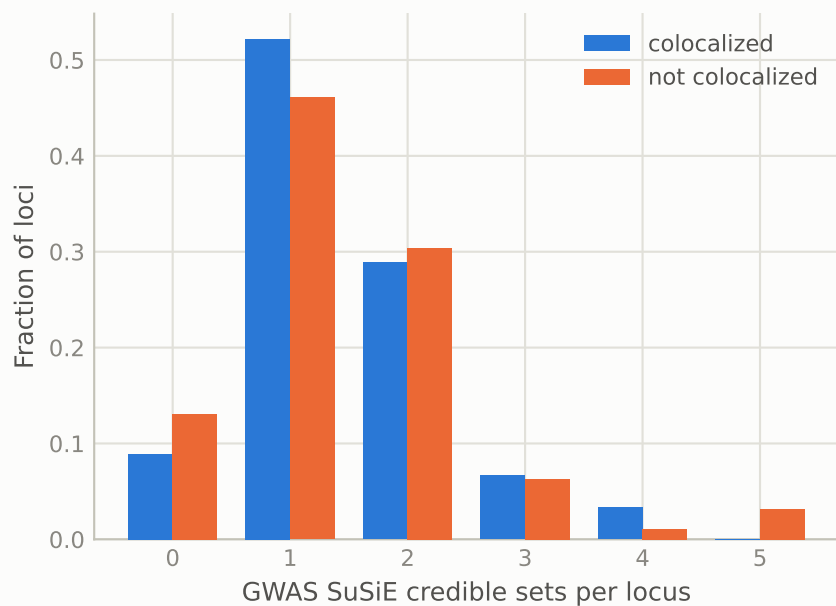
C Allelic heterogeneity (multi-CS Fisher p=0.8 )
