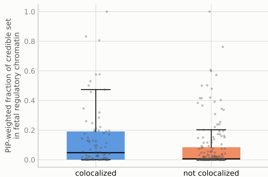
D Fetal regulatory annotation (MWU p=0.0011 )
