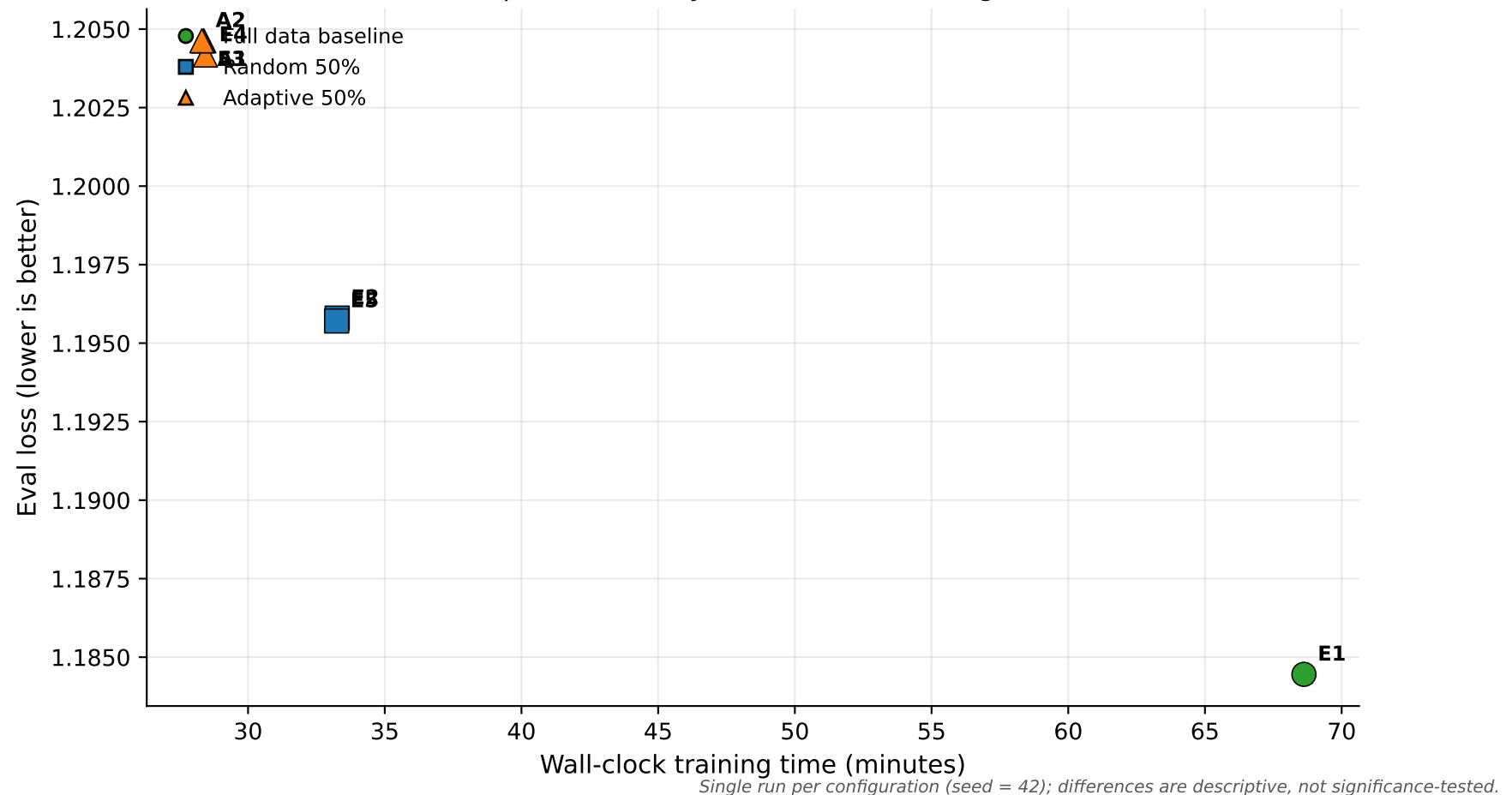
Compute efficiency: eval loss vs training time
