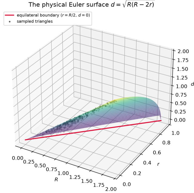
FIGURE 1. The physical Euler surface d = \sqrt{R(R - 2r)} over \{R > 0, 0 < r \leq R/2\} , with 600 sampled triangles (black dots) lying exactly on it. The red line is the equilateral edge r = R/2, d = 0 .
