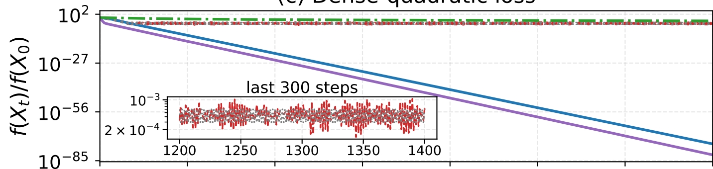
(c) Dense-quadratic loss
