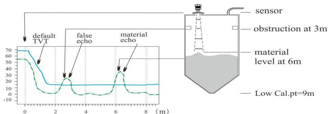
Example before Auto False Echo Suppression
