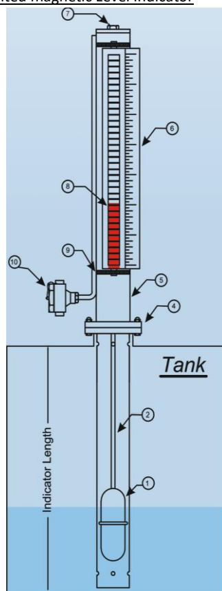
TOP Mounted magnetic Level Indicator
