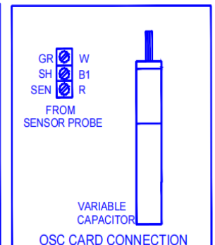
Oscillator Card
