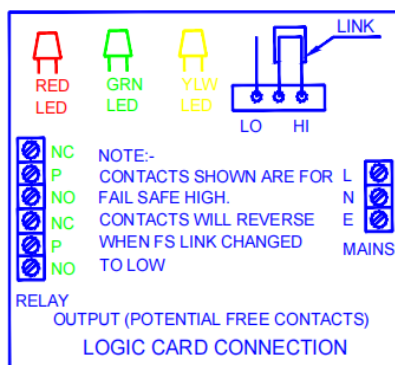
Controller Card
