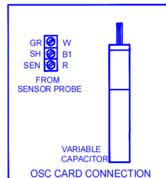
Oscillator Card
