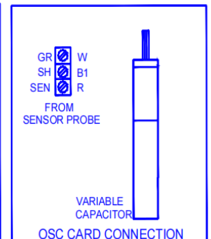
Oscillator Card
