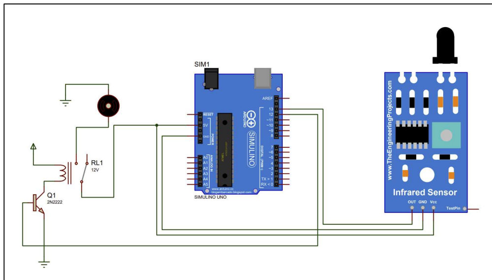
Circuit (b): IR sensor and relay connections with Arduino UNO
