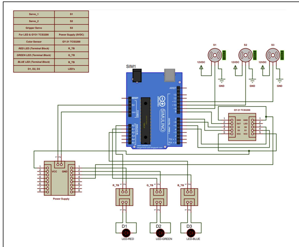
Circuit (a) Colour sensor and Motor connections with Arduino UNO
