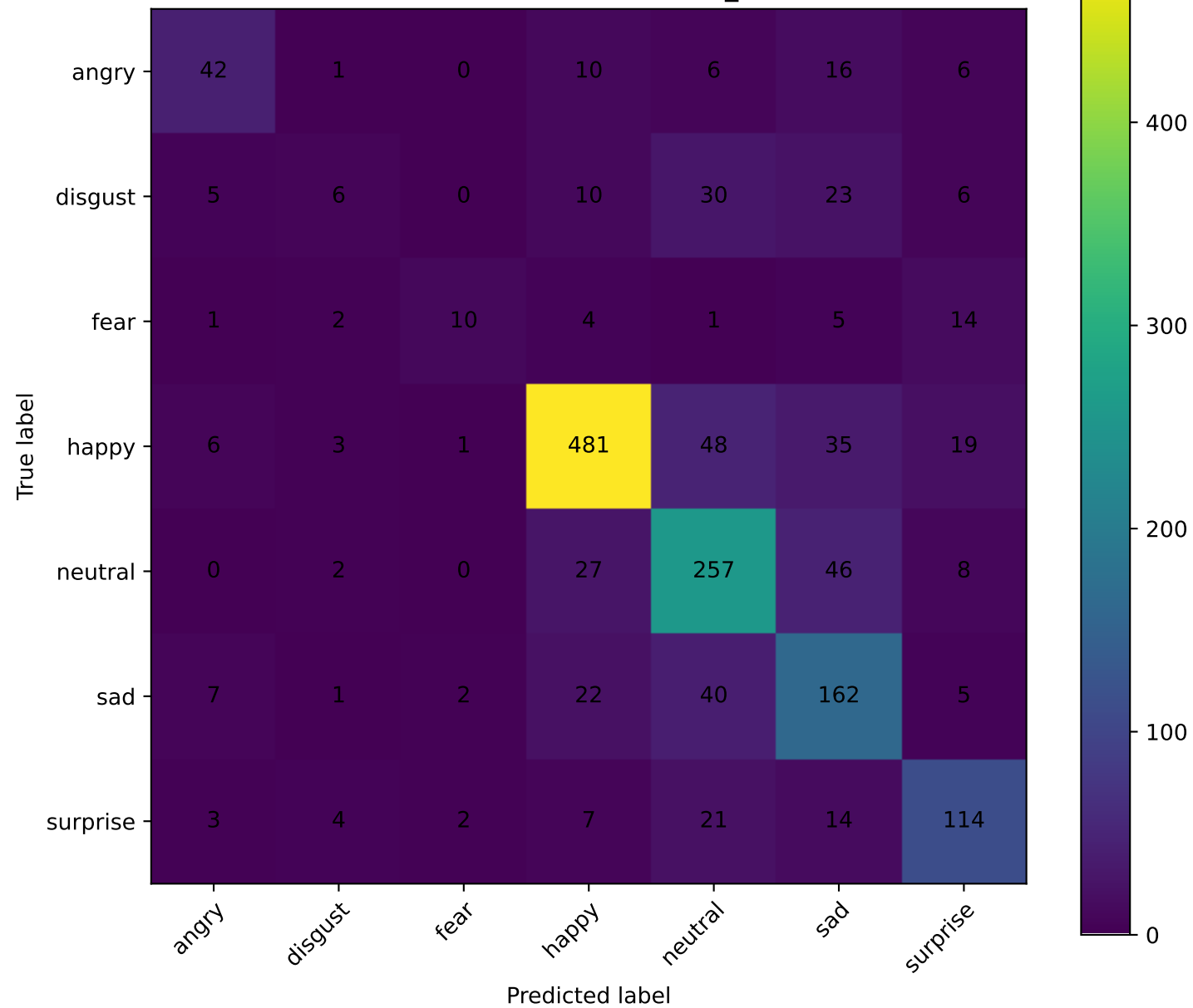
Confusion Matrix: Custom_CNN
