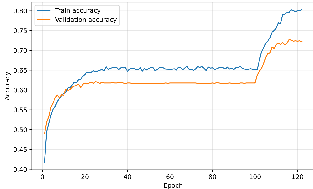
MobileNetV2: Accuracy
