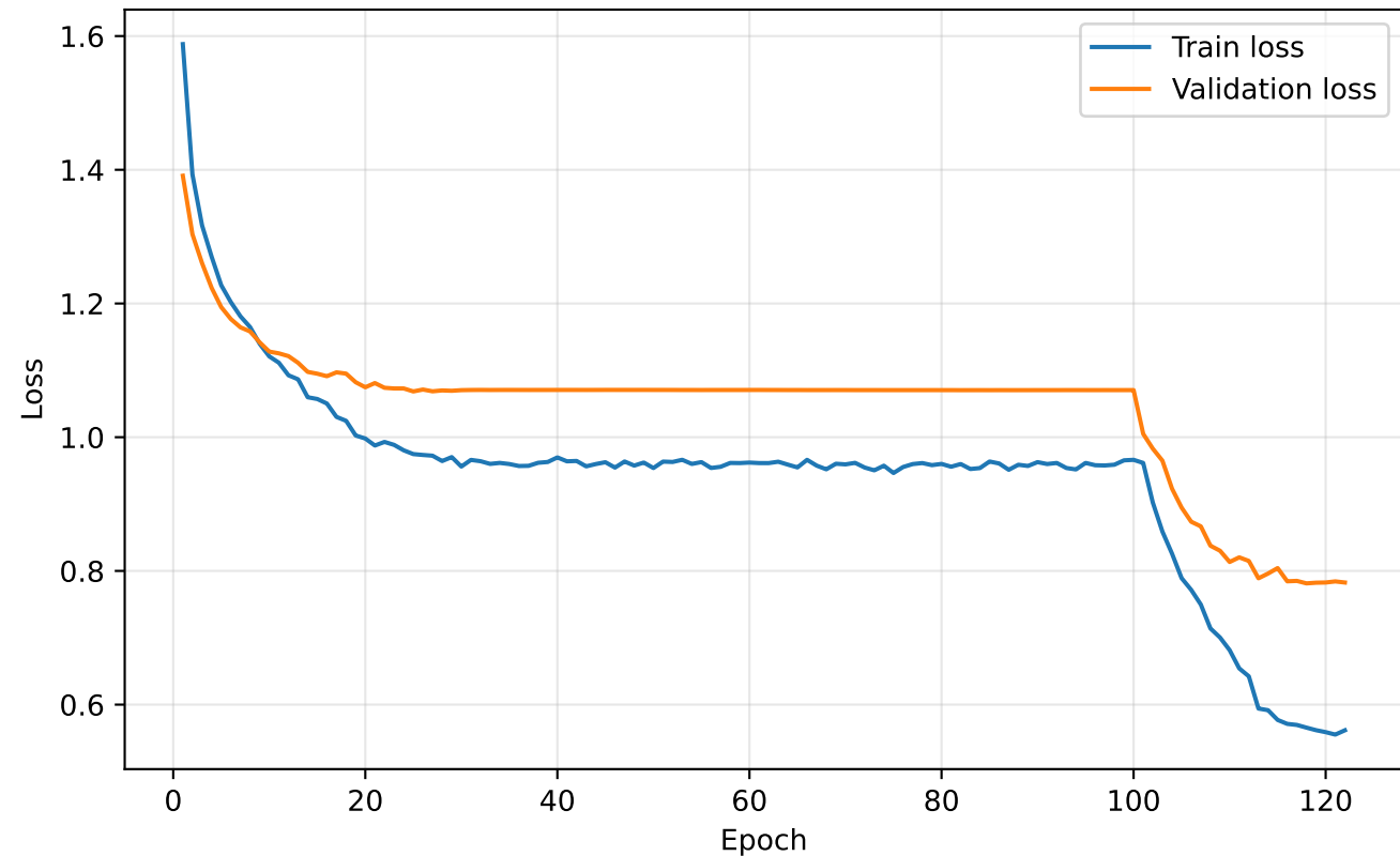
MobileNetV2: Loss
