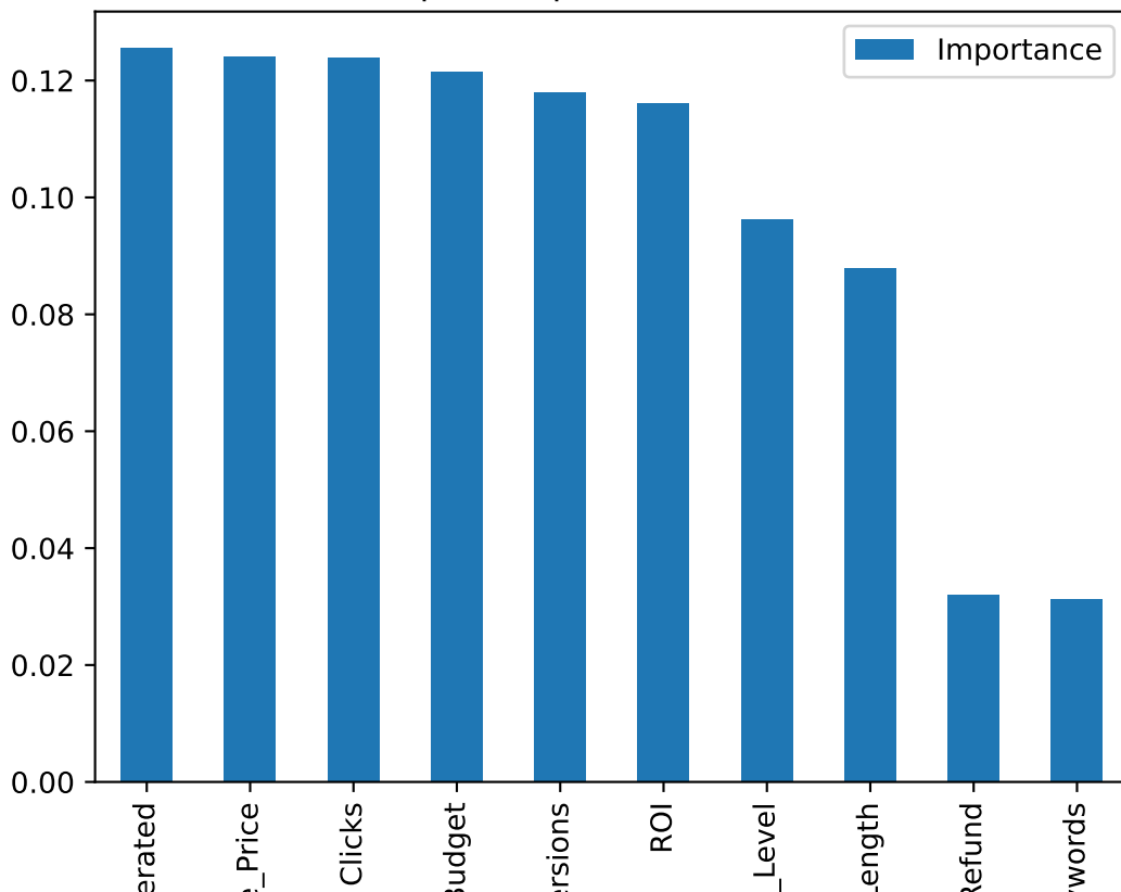
Top 10 Important Features
