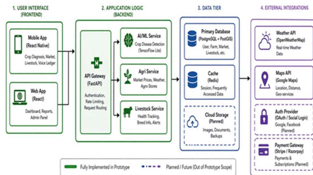
Fig. 1: KisanShakti System Architecture and Prototype Scope Overview
