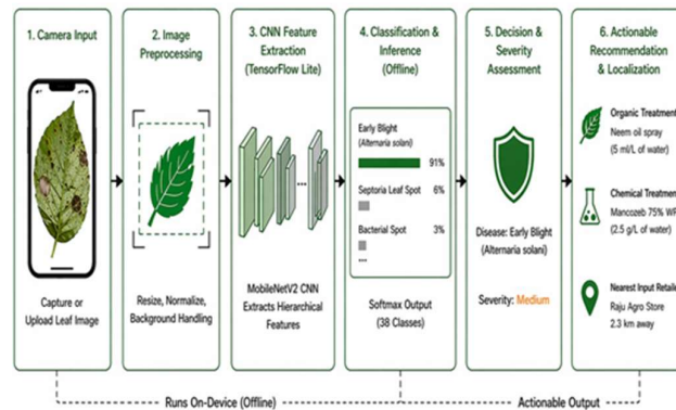
Fig. 2: AI-based crop disease detection workflow
