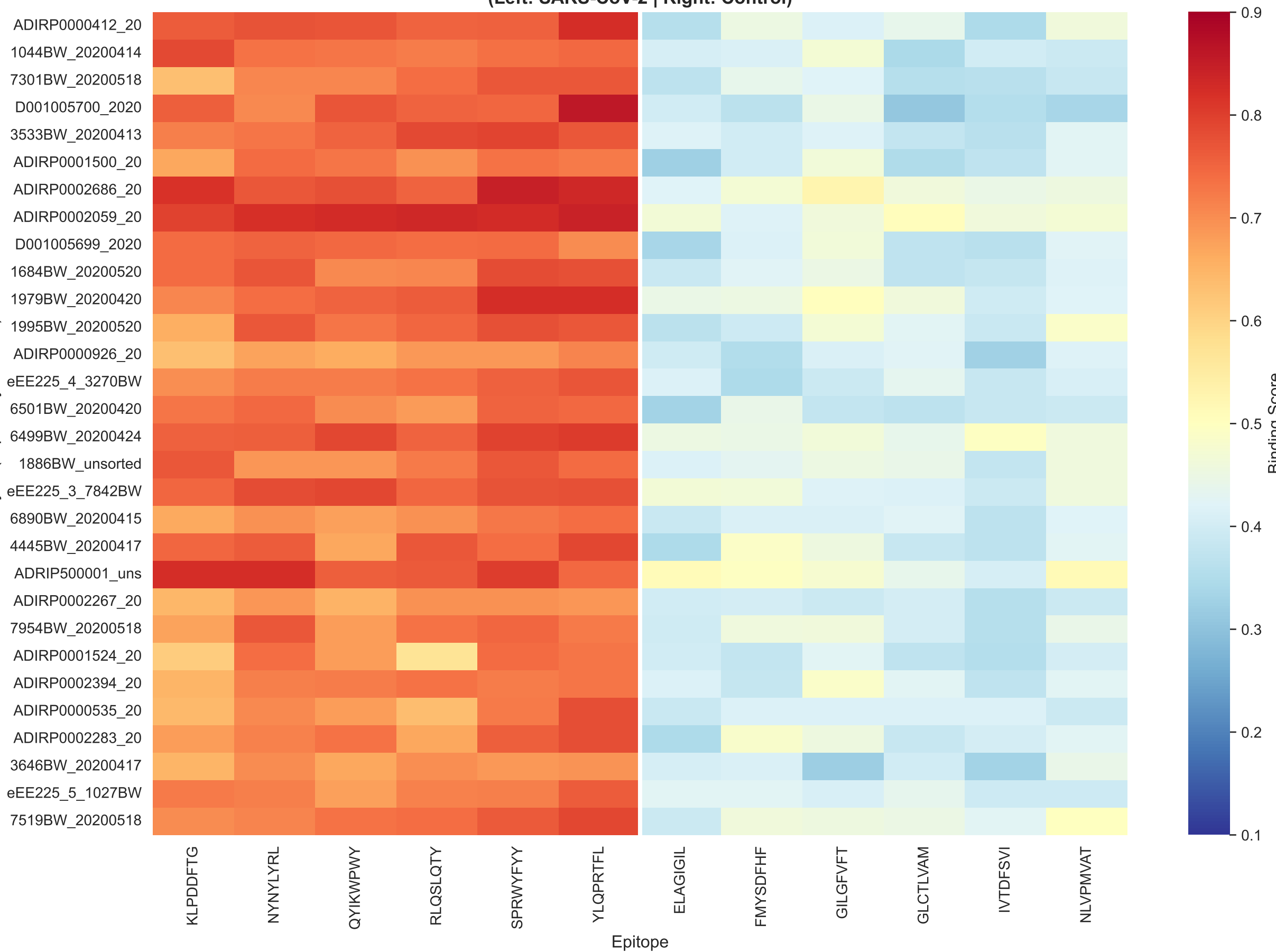
Subject × Epitope Binding Score Heatmap (Left: SARS-CoV-2 | Right: Control)
