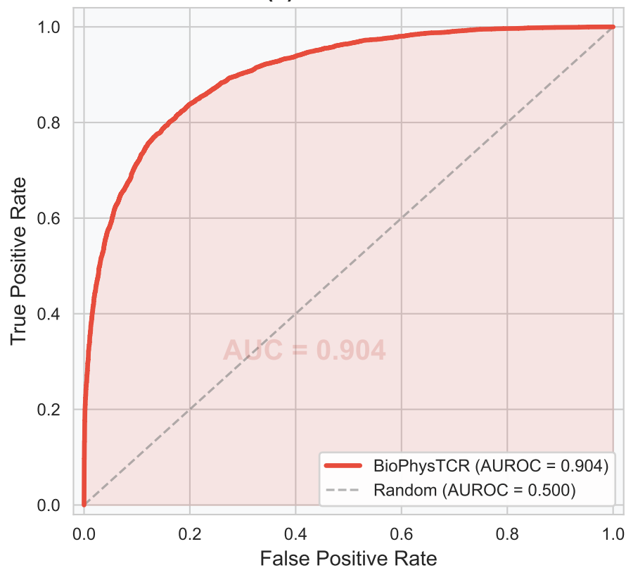
(a) ROC Curve
