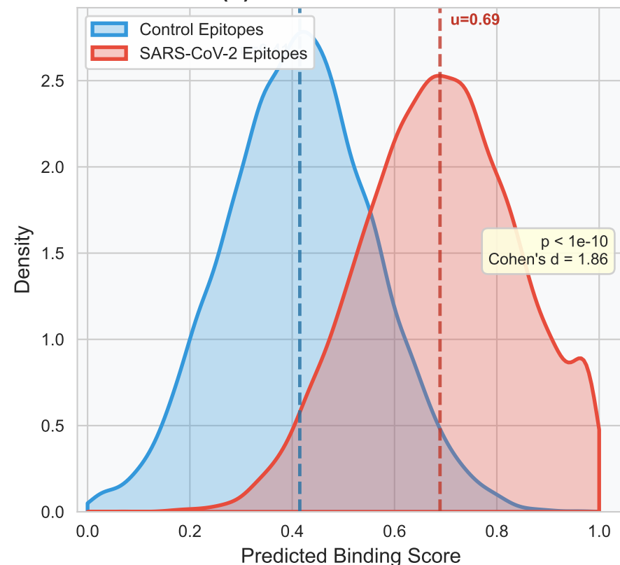
(b) Score Distributions
