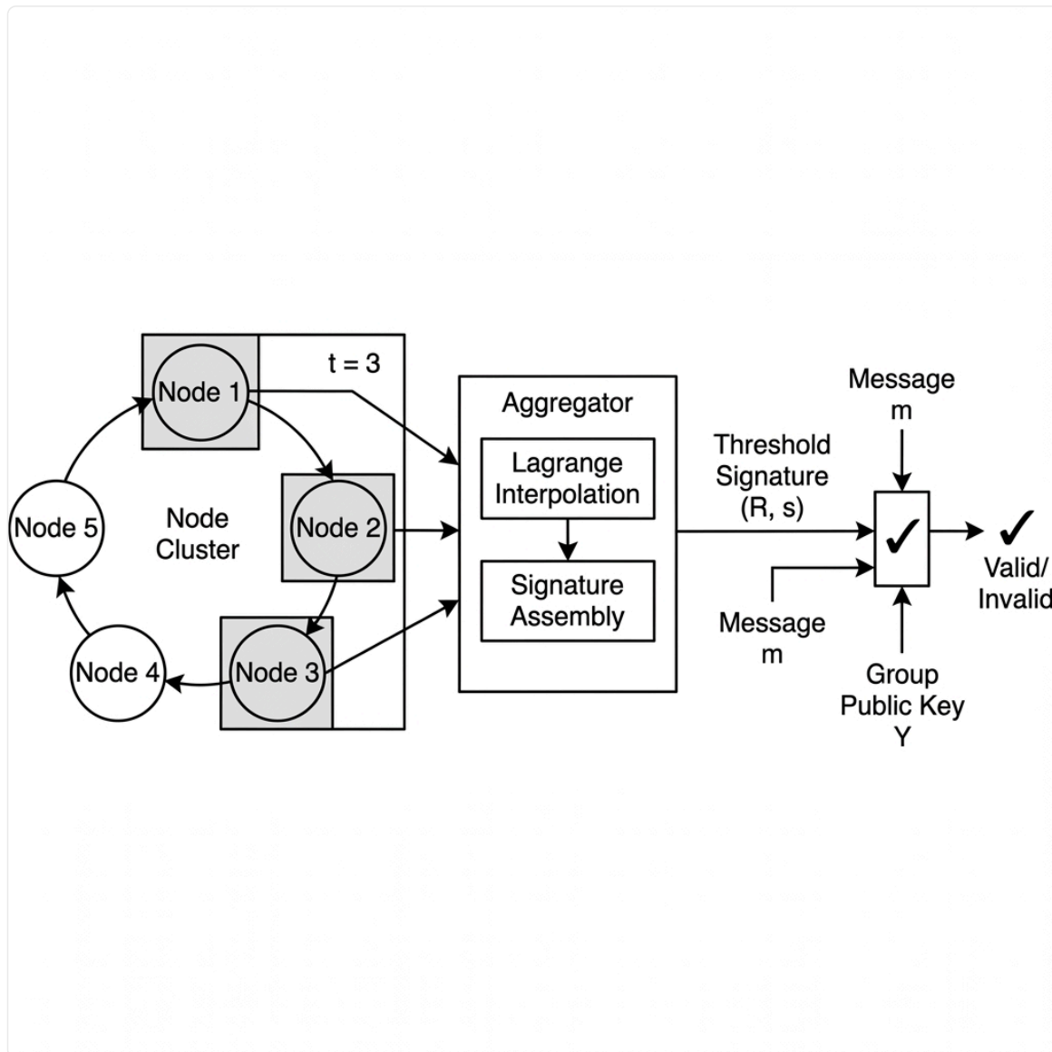
Figure 3: Threshold MPC Signing Process Subset of t participants generate partial signatures using Lagrange interpolation, aggregated into a single threshold signature verified against the group public key.
