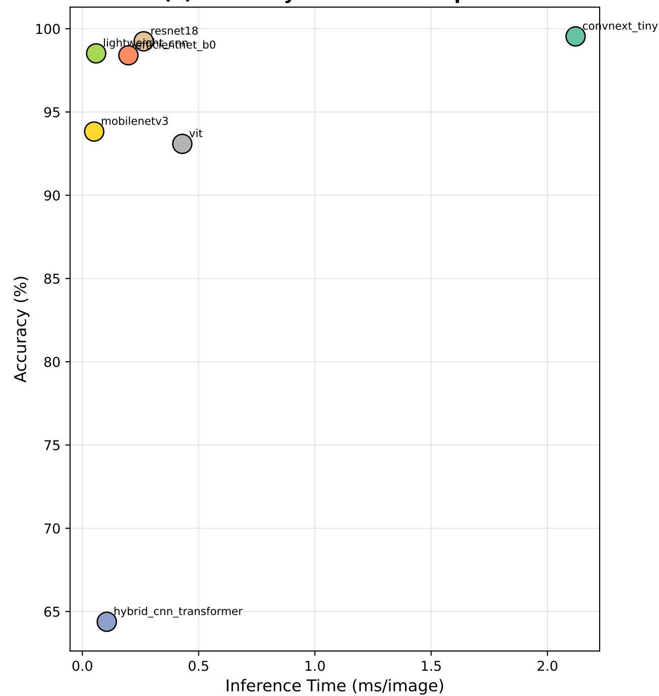
(e) Accuracy vs Inference Speed
