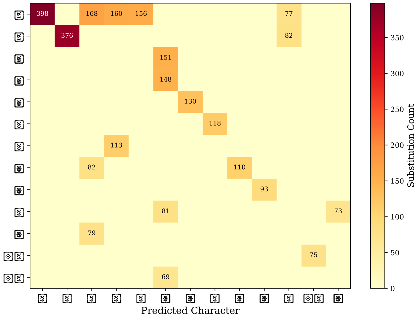
Character Confusion Matrix — CTC Model
