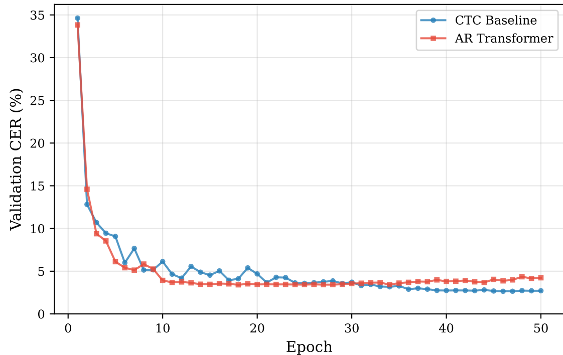
(a) Character Error Rate
