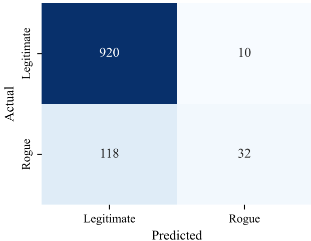
Confusion Matrix (Baseline QTK)
