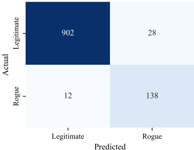
Confusion Matrix (Proposed Dual-Trigger QTK)
