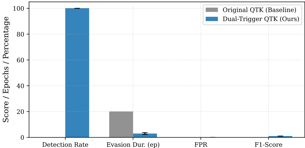
RQ1: Original QTK vs. Dual-Trigger QTK Performance
