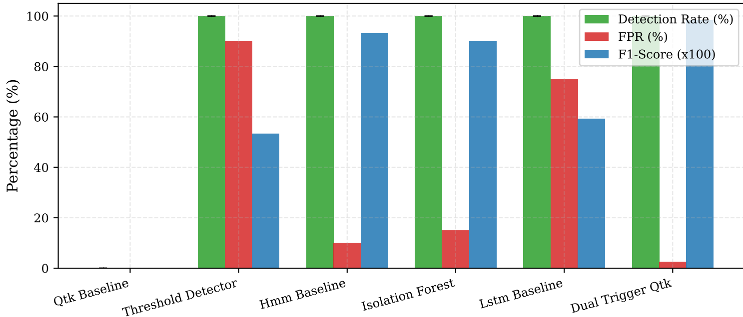
Behavioral Baselines Comparison on Test Workload
