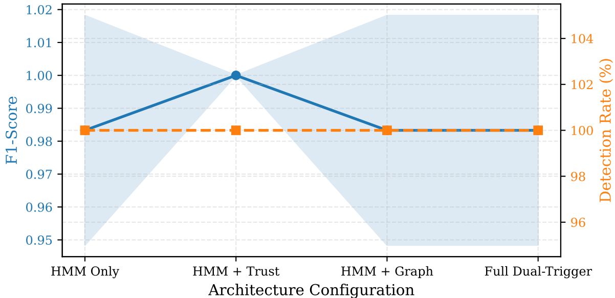
RQ2: Component Ablation Analysis
