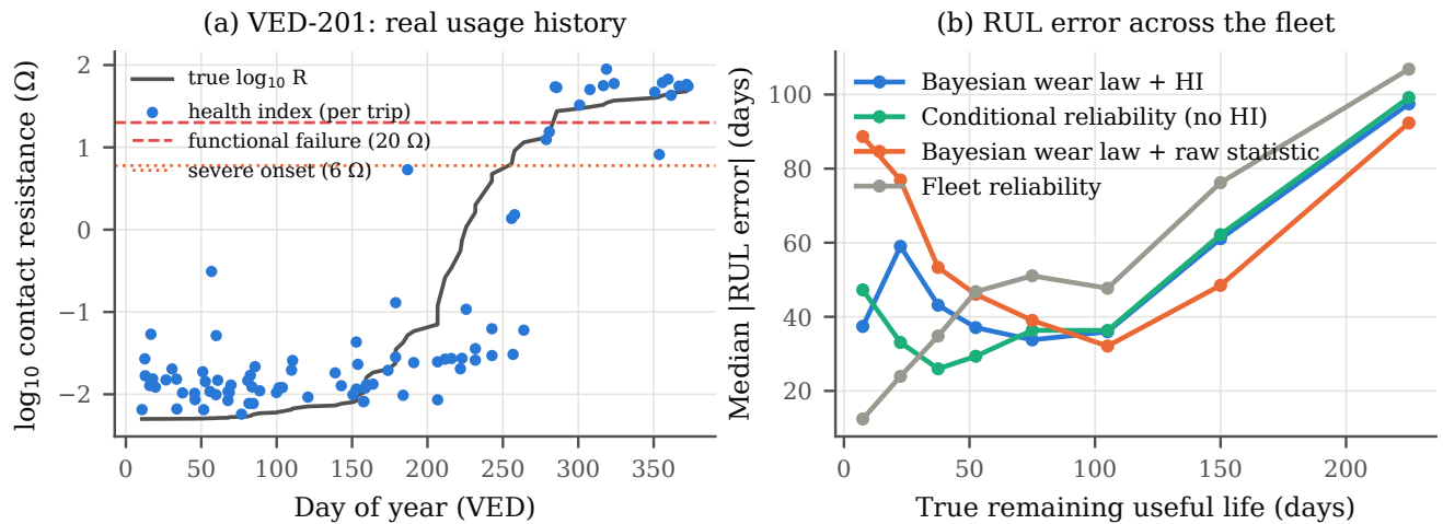
FIGURE 6. Fleet prognosis on VED. (a) One vehicle's connector, wearing with its own recorded usage: true resistance and the per-trip health index learned from telemetry by a vehicle-disjoint model. (b) Median absolute RUL error versus true RUL across all failing vehicles ( 20\text{-}\Omega failure definition; the trend alarm is not a point estimator and is omitted).
