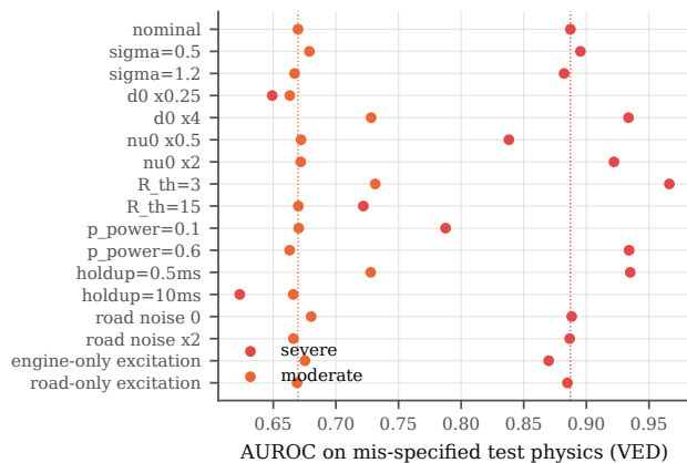
FIGURE 7. Robustness of VED detection when the test data are generated with mis-specified physics (training always uses the nominal model of Table 1). Dotted lines: nominal test physics. AUROC against healthy and confounder trips; held-out half of the vehicles.
