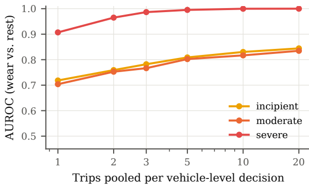
FIGURE 5. Vehicle-level detection on VED when the per-trip log-odds of K trips of the same vehicle are averaged. Negatives include healthy and all confounder trips.
