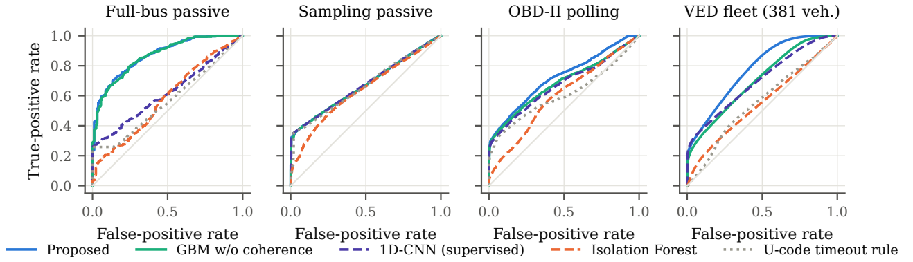
FIGURE 3. ROC curves (wear vs. healthy and confounders) on the four corpora, pooled out-of-fold scores.
