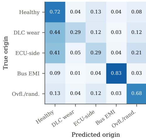
FIGURE 4. Row-normalized attribution confusion matrix, VED fleet (381 vehicles, vehicle-disjoint folds).
