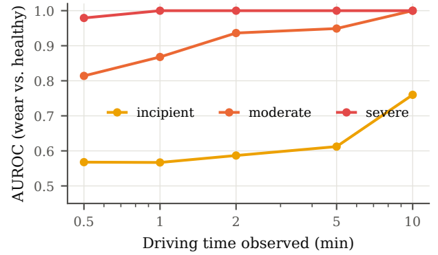
FIGURE 4. Full-bus detection when one persistent fault is applied to an entire real drive and the evidence of consecutive 30-s windows is accumulated (vehicle-disjoint models). Points are shown while at least 50 drive trajectories are long enough (399 at 0.5–2 min, 252 at 5 min, 105 at 10 min).
