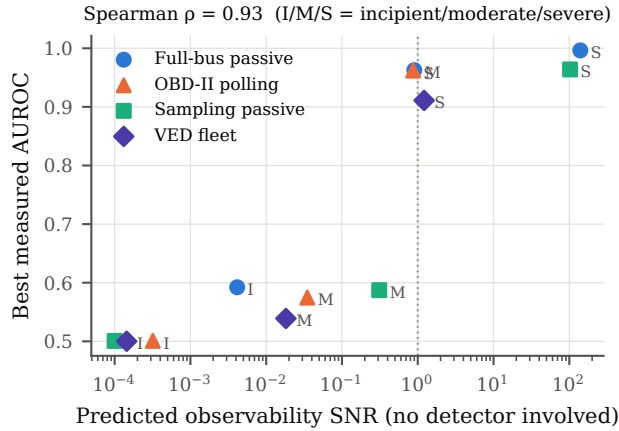
FIGURE 3. Predicted observability SNR (Section IV-E), computed from the physics and each tool's measured healthy background without any detector, against the best AUROC measured for that tool and stage (I, M, S: incipient, moderate, severe wear).
