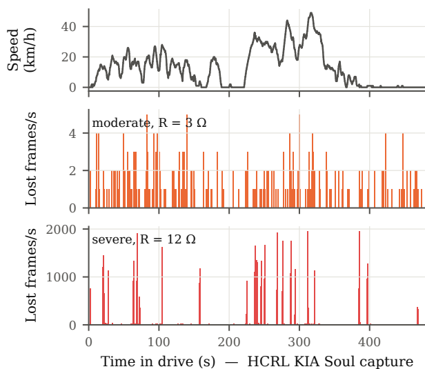
FIGURE 2. A real 8-minute drive of the HCRL KIA Soul (top: decoded vehicle speed) replayed through a moderately (middle) and severely (bottom) worn DLC. Losses cluster where the vehicle is moving and vanish at standstill: the excitation coherence that ECTA measures. Severe wear adds brown-out silences (tall bars).
