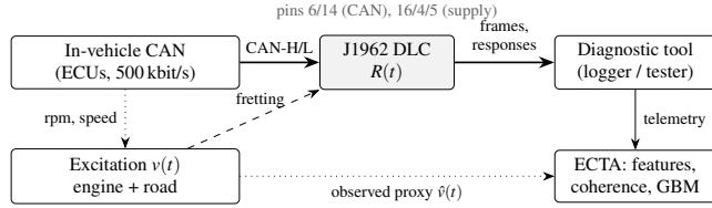
FIGURE 1. Problem setting. Vibration excitation v(t) drives fretting of the DLC contacts and modulates their interruption rate. The tool observes only its own telemetry, from which ECTA also recovers an excitation proxy \hat{v}(t) .
