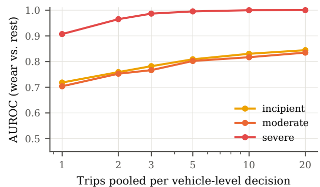
FIGURE 7. Vehicle-level detection on VED when the per-trip log-odds of K trips of the same vehicle are averaged. Negatives include healthy and all confounder trips.
