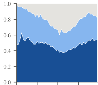
EDF-Threshold
