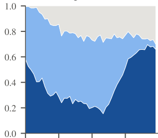
Cog-Heuristic
