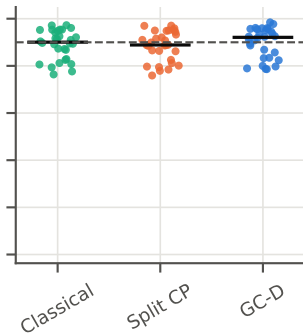
Soil: new region (30 groups)
