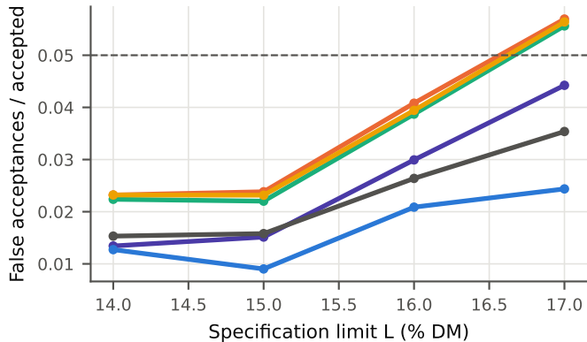
(a) Wrongly accepted ' DM \geq L ' decisions
